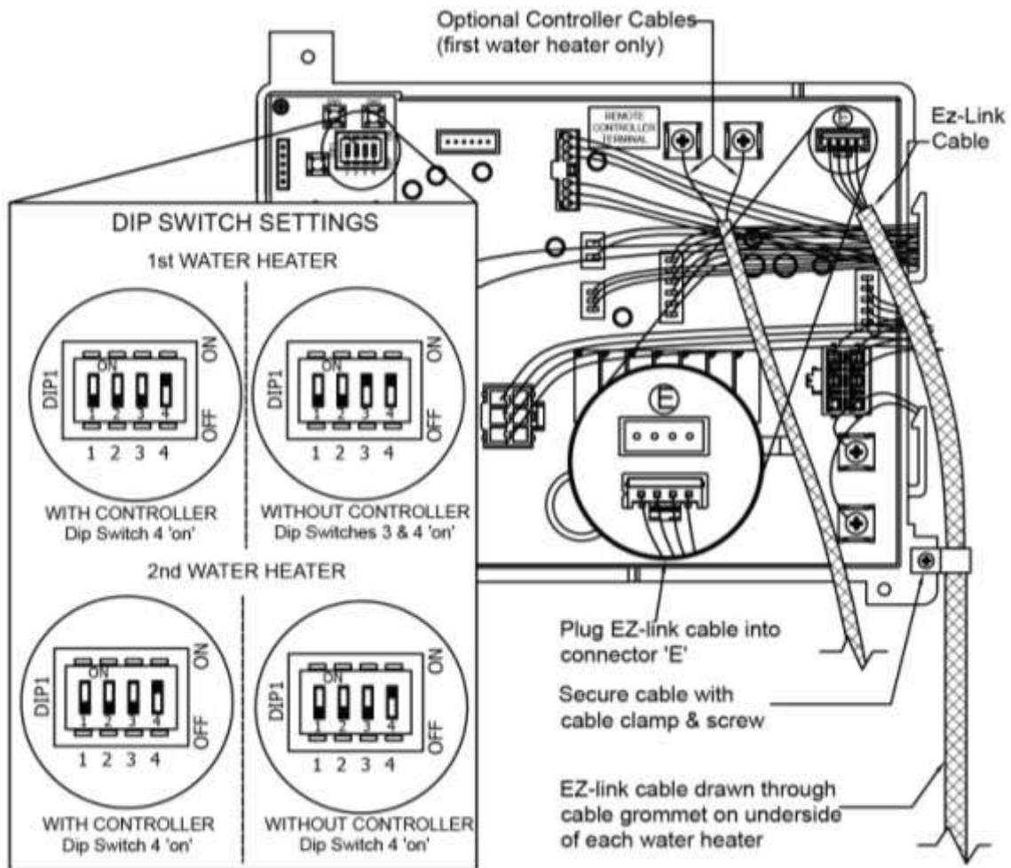
Control Board with Ez-Link Connection 874 and 876 series 612, 616, E16, 618 and 620 models
