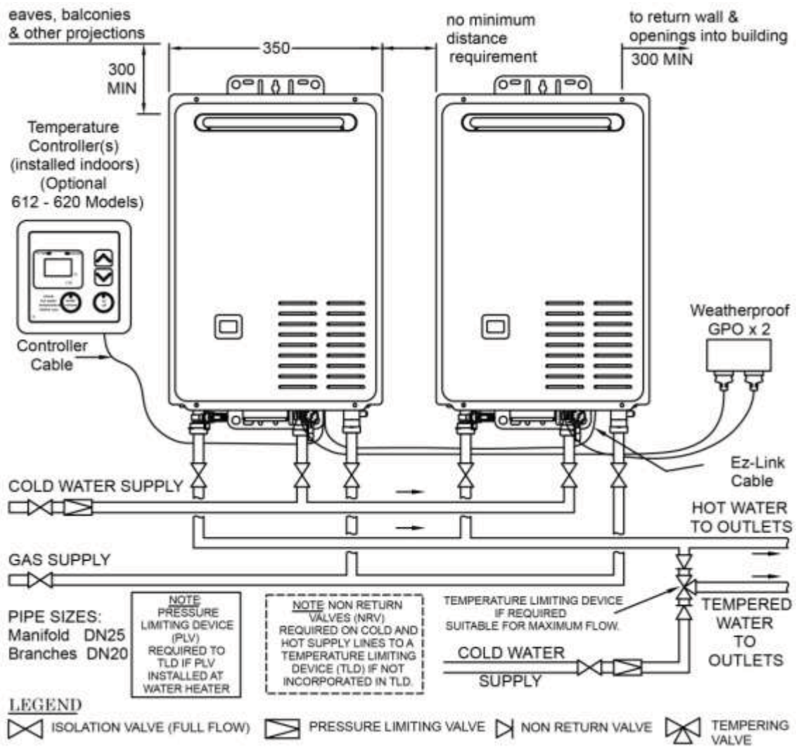
Typical Two Unit Manifold with Ez-Link Connection 874 and 876 series 612, 616, E16, 618 and 620 models
