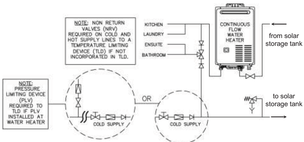
In-series Gas Booster as part of a Closed Circuit Indirect Solar Water Heater Installation Two Temperature Zones Using a Temperature Limiting Device
