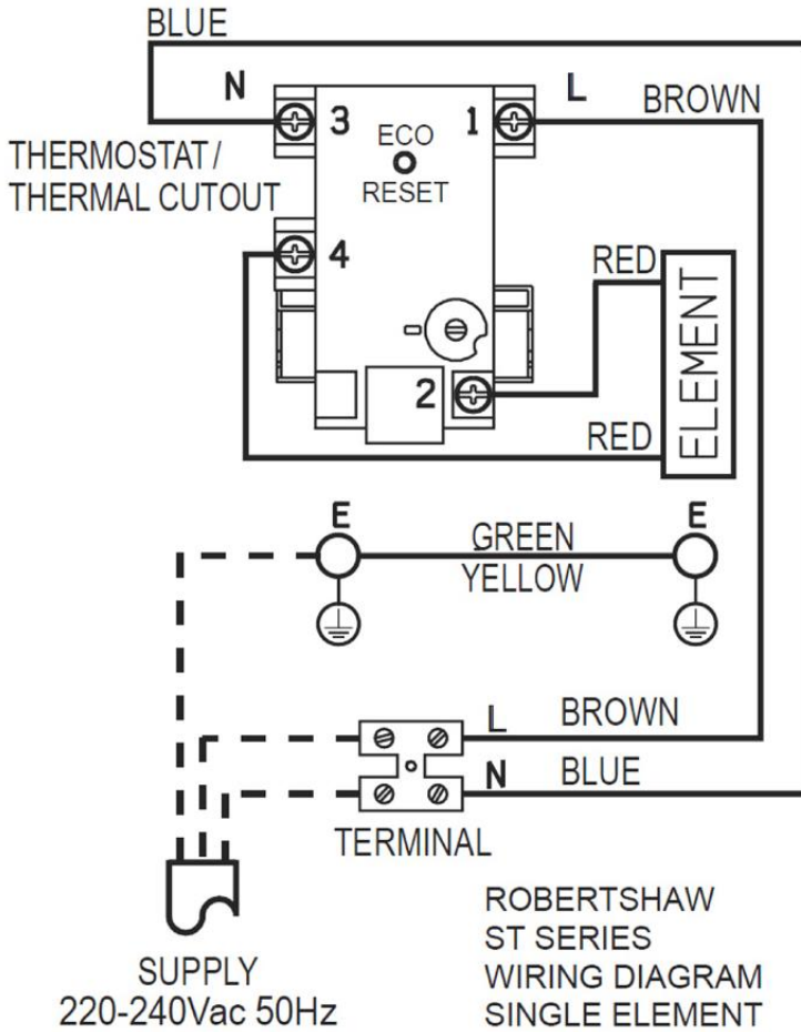
Electrical Circuit for Single Element Models – Robertshaw “ST” Thermostats
