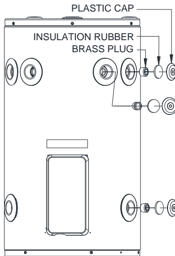
025, 045, 050 models
