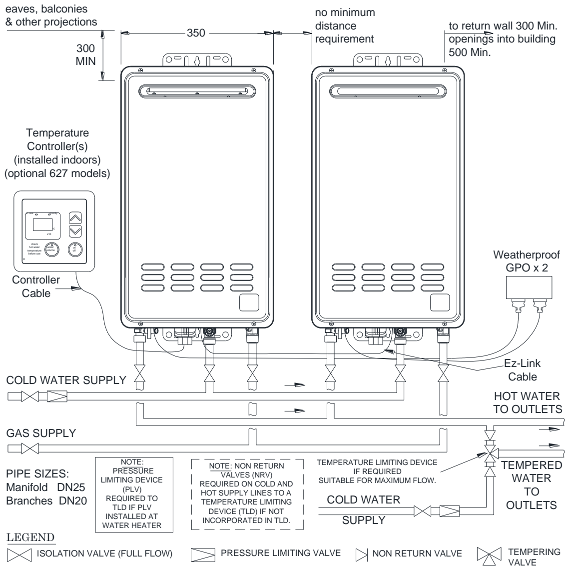
Typical Two Unit Manifold with Ez-Link Connection
