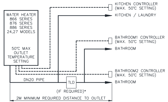
876 Series – Kitchen and Bathroom Controllers
