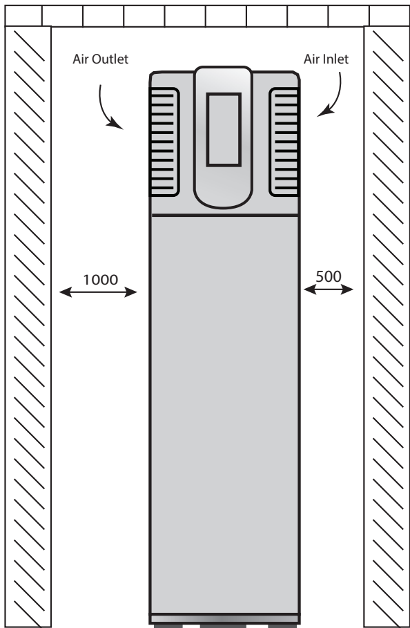
Diagram 2b. Front View Unit: mm
