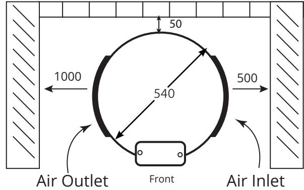
Diagram 2a. Top View Unit: mm
